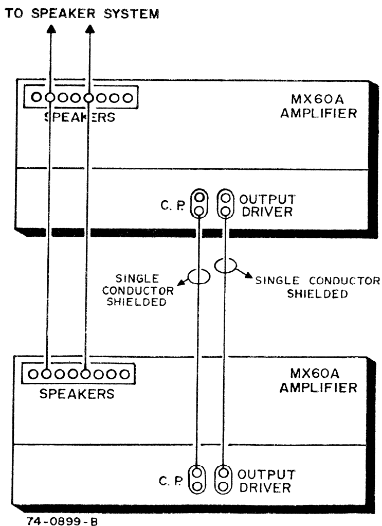
Figure 7 - Paralleling Amplifiers
